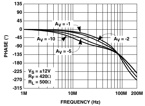
FIGURE 6. INVERTING FREQUENCY RESPONSE (PHASE)
