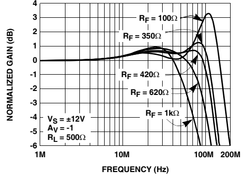
FIGURE 2. INVERTING FREQUENCY RESPONSE FOR VARIOUS R_F
